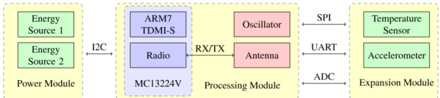
EPOSMote II block diagram
